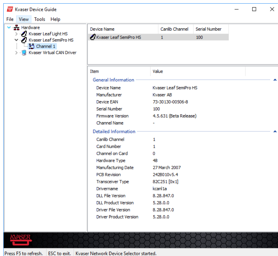
Figure 4: Channel information
